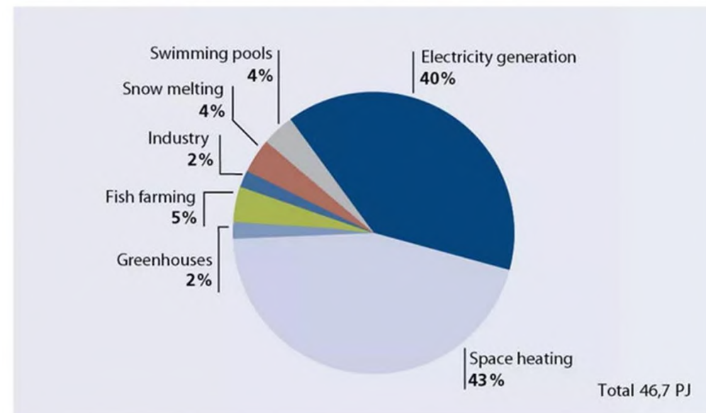
Utilisation of geothermal energy 2013
